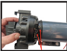
6. Place pump head on shaft of motor and rotate until the set screw holes are beside each other as shown above.
