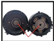
5. Locate the straight spot on both the motor and replacement head. These parts will mate with each other.
